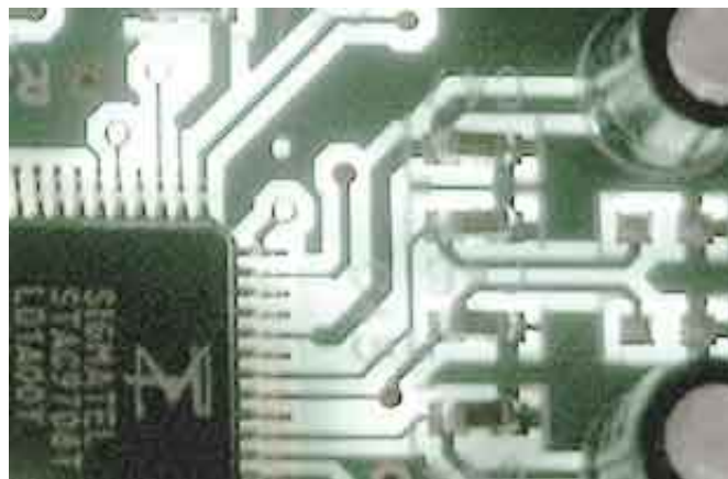
Direct3d 9 Windows 7
